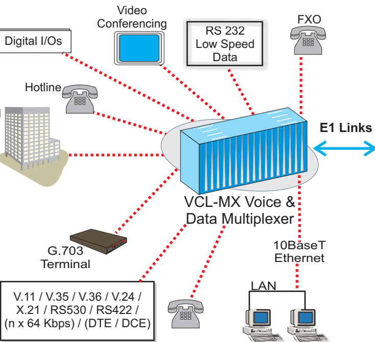
VCL-MX, E1 Multiplexer Interfaces Cards - Voice and Data applications
